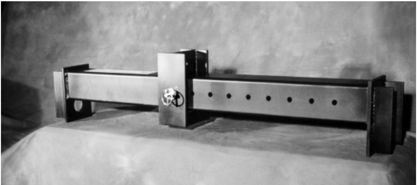
Figure 1. The V-DOSC Spreader
