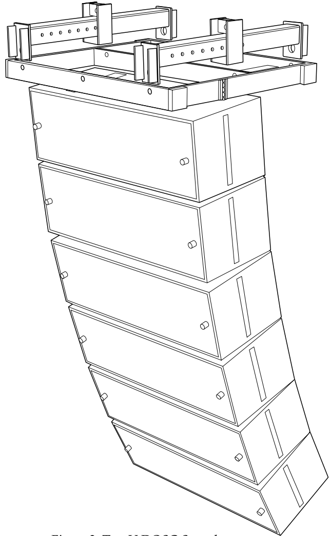
Figure 3. Two V-DOSC Spreaders used to provide low head room side by side support for a standard V-DOSC rig.
