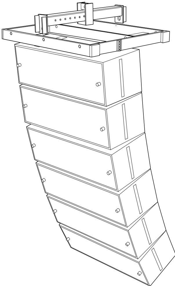
Figure 2. One V-DOSC Spreader used to provide low head room single point support for a standard V-DOSC rig.
